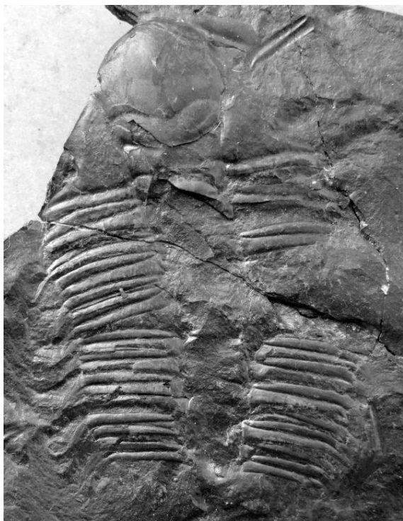
Hydrocephalus minor Boeck, 1827 †
