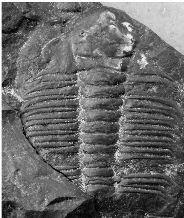
Hydrocephalus minor Boeck, 1827 †
